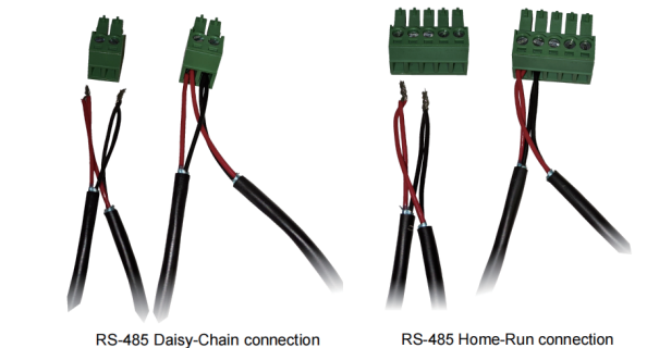
RS-485 Daisy-Chain connection
